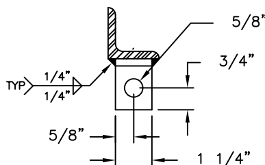
BOLT TAB DETAIL
